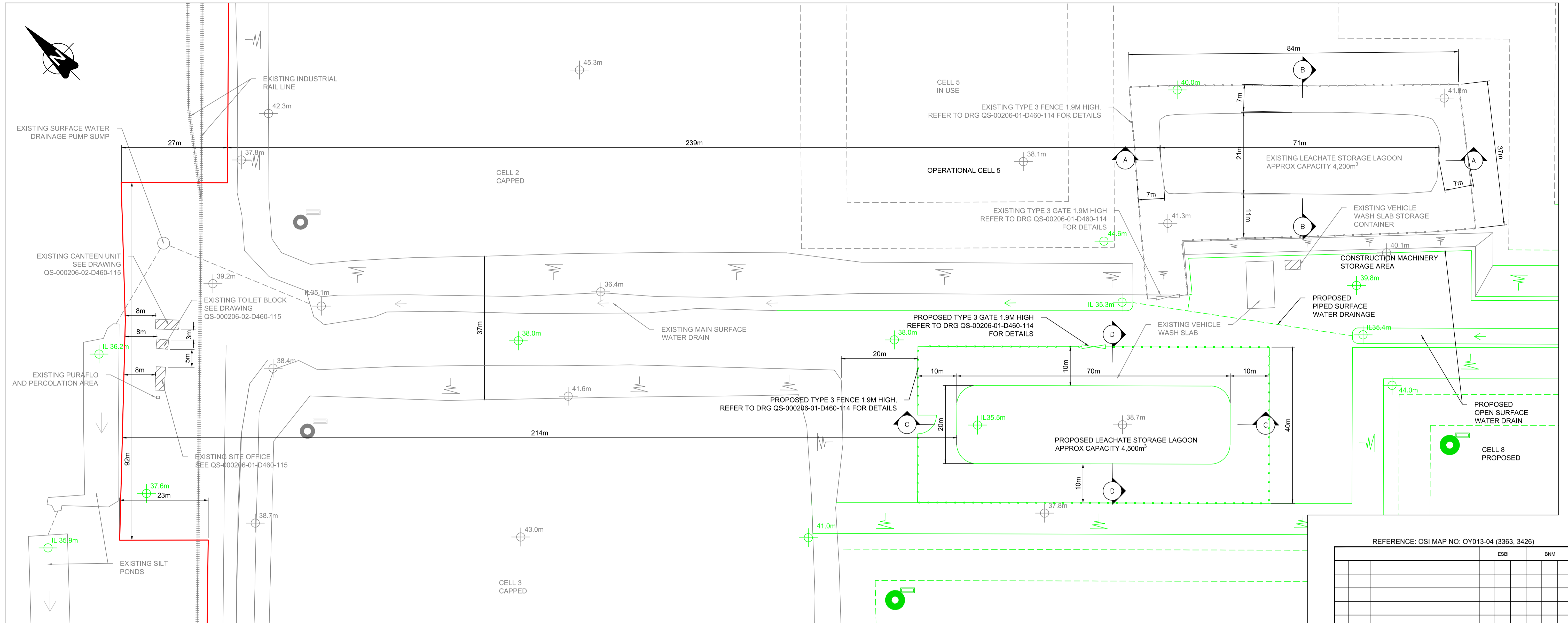
PLAN SCALE 1:500
